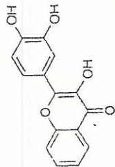
3,3',4'-Trihydroxy Flavone
